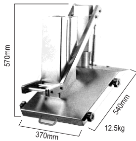
Cheese (or single) feeder 12.5kg
