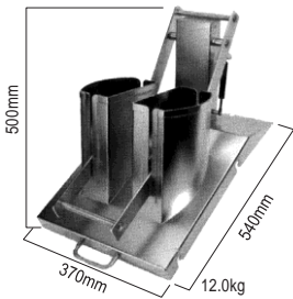
Double Feeder (used with MC double blade sets) 12.0kg
